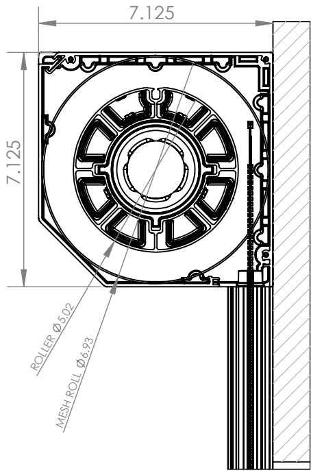
7.125" HOUSING ASSY SECTION VIEW SCALE 1:4
