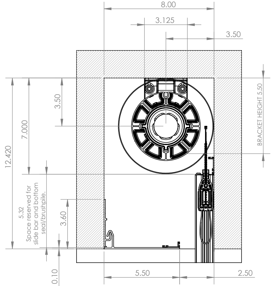
VERTICALLY MOUNTED BRACKETS
