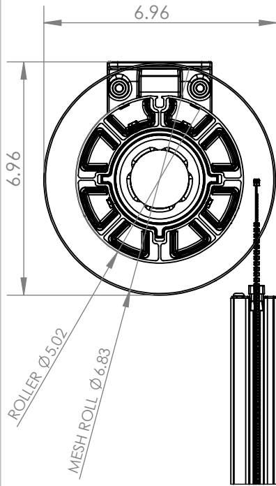
5" RECESSED ROLLER ASSY SECTION VIEW SCALE 1:4
