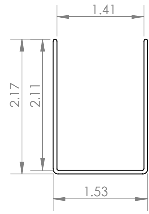
U-GUARD TOP VIEW SCALE 1:1.5
