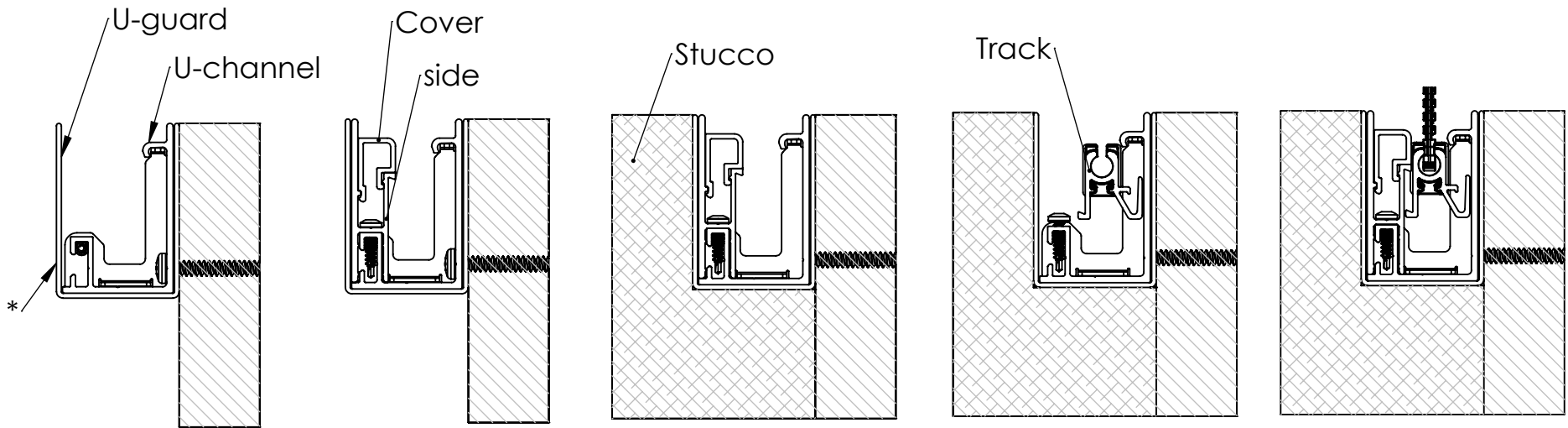
(A) Mount U-channel and U-guard
