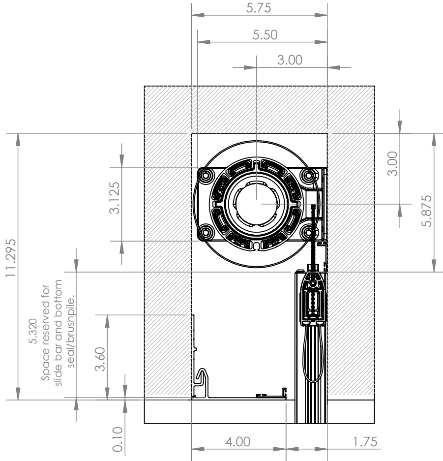
HORIZONTALLY MOUNTED BRACKETS
