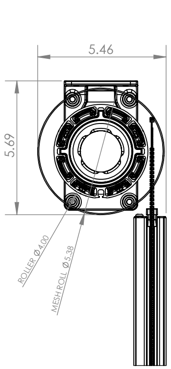
4" RECESSED ROLLER ASSY SECTION VIEW SCALE 1:4
