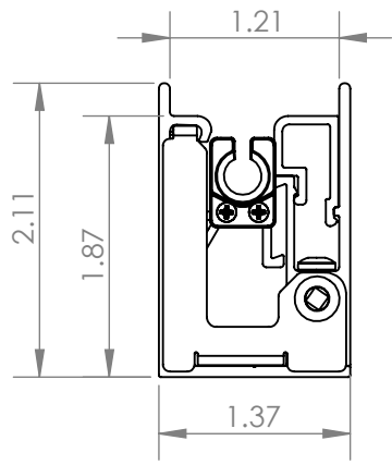
SURE FIT TRACK ASSY TOP VIEW SCALE 1:1.5
