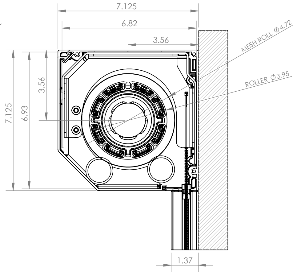
Mz1.0 Carrier
