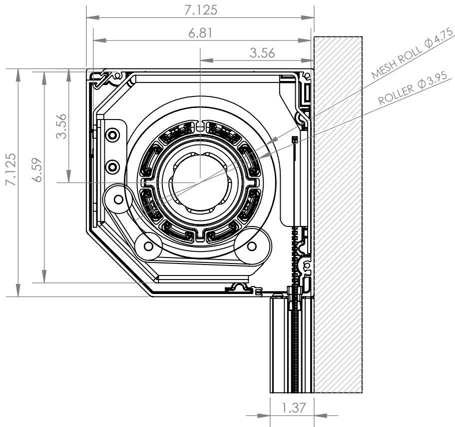
Mz2.0 Carrier
