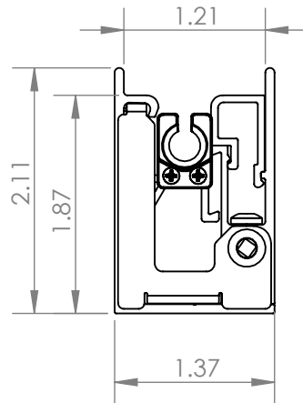
SURE FIT TRACK ASSY TOP VIEW SCALE 1:1.5
