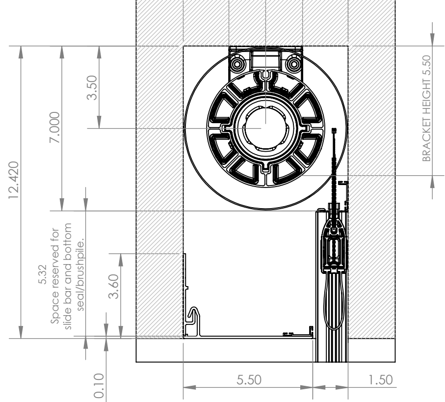
VERTICALLY MOUNTED BRACKETS
