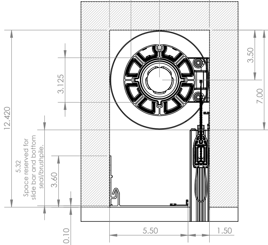
HORIZONTALLY MOUNTED BRACKETS
