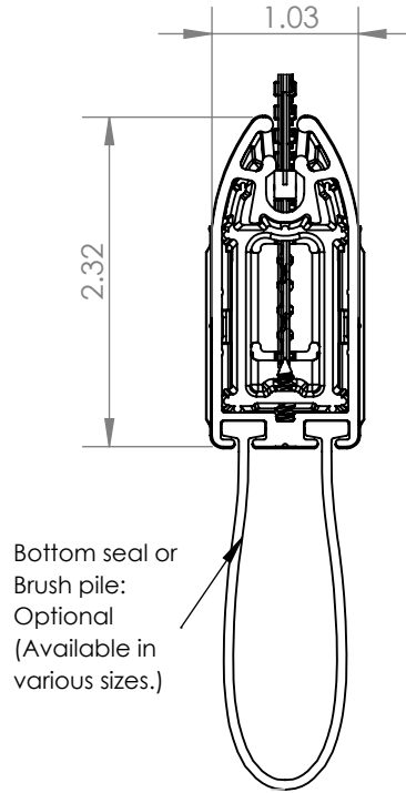
SLIDEBAR ASSY SECTION VIEW SCALE 1:1.5
